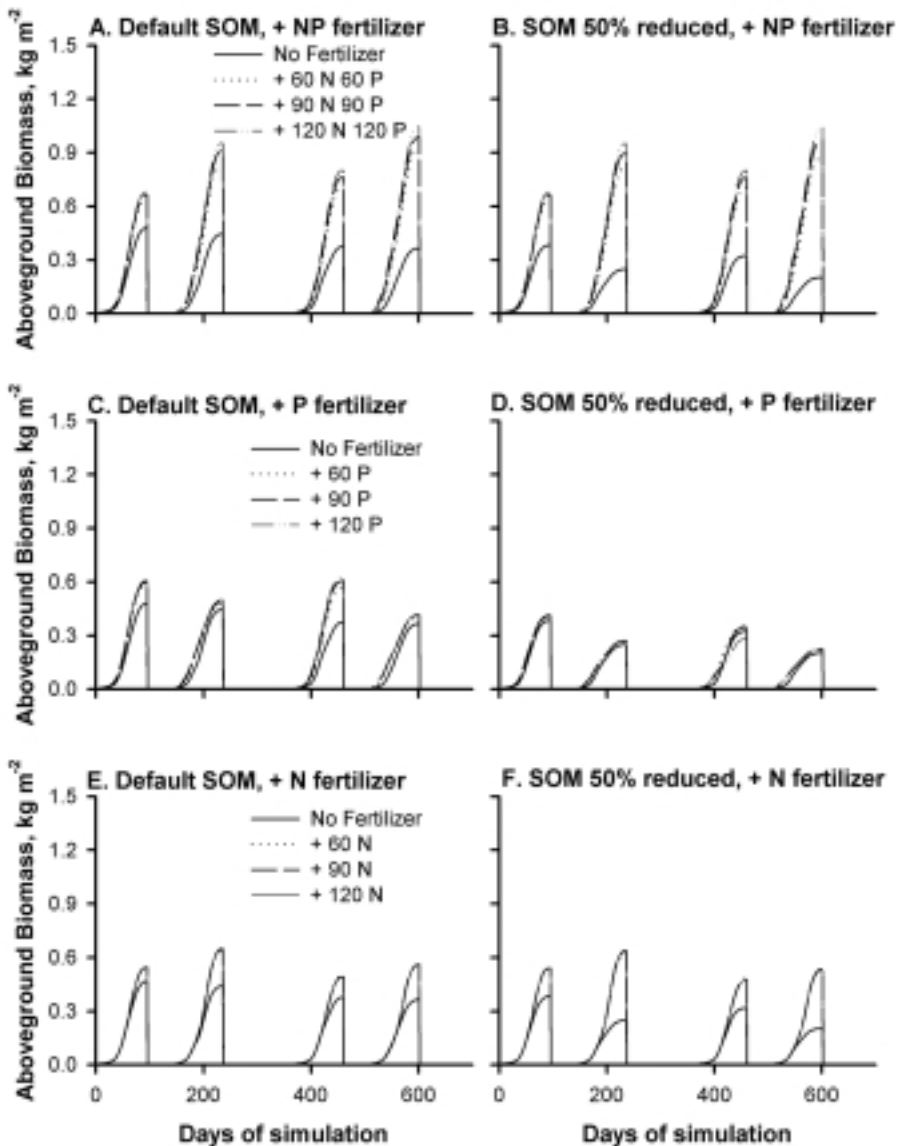
Figure 4.3 A..F. Simulated crop development (total aboveground biomass) for maize with a Lampung climate and default parameters setting (for changes in parameter settings from the default values, see Table 4.1), with or without N fertilizer (at 60, 90 or 120 kg N ha -1 crop -1 , with split application (50% at planting, 50% at 30 days later). We also used the same amounts for P fertilizer; it is applied once at planting time. The simulation also knows the impact of reducing 50% of soil organic matter content.
