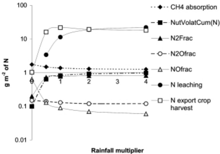
Figure 3.15. Effect of total rainfall, as simulated by using multiplier on daily rainfall amounts, on the gaseous N emissions from a soil (specified over NO and N 2 O), leaching and N export from the plot in crop harvests over a 5 year period
