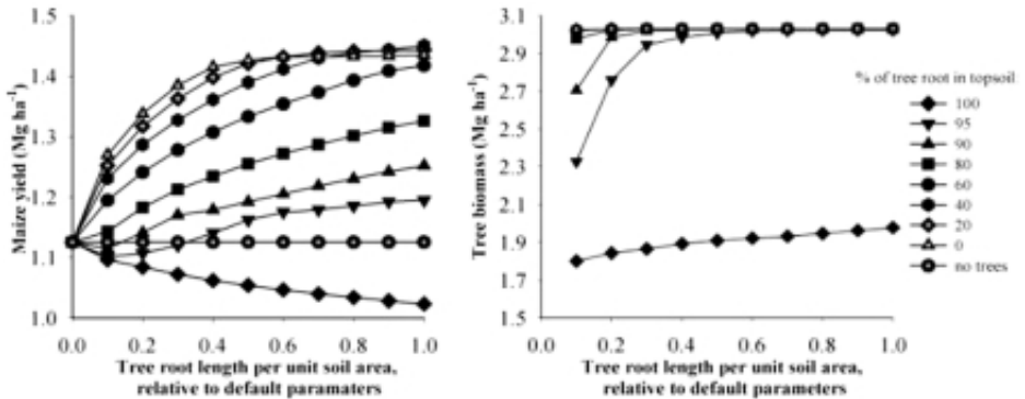
Figure 4.18 Predicted maize yield (A) and tree biomass (B) for the default rainfall situation (2318 mm year -1 ), when relative distribution of tree roots with depth as well as total amount of tree roots are varied independently. Whereas the 'default' tree roots system had 21.5% of its roots in the top layer, a series of data was made that had 0 - 100% of its roots in the top layer and the remainder allocated to the deeper layers in proportion to the root length densities of the default case (the relative distribution over the four zones with increasing distance to the tree was not modified). For each of these root distributions, the total amount of roots was varied from 0.1 - 1 times the default, while maintaining the relative value.
