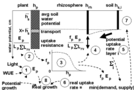
Figure 3.6. Steps (1...8) in daily cycle of calculations of water uptake; the interrupted arrows represent information flows
