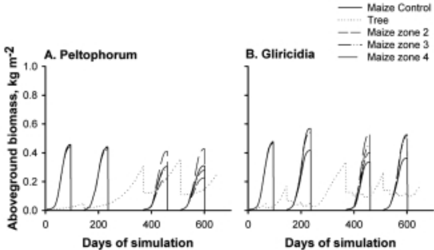
Figure 4.4 Model predictions with WaNuLCAS 3.0 of development of hedgerow tree canopy and crop biomass (on a whole field basis) over four cropping seasons in two years, for three crop zones (2, 3 and 4) within the alleys (the P and G trees approximate Peltophorum and Gliricidia, respectively, as used in experiments in Lampung (Indonesia); van Noordwijk et al. , 1998a); zones 2, 3 and 4 are 1 m wide each; soil type, rainfall pattern and potential maize production inputs were derived from the Lampung site
