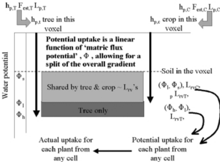
Figure 3.7. Diagram of sharing out available water by tree and crop
