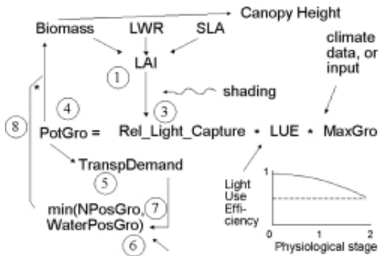
Figure 3.21. Major relationships in the daily cycle of calculating crop biomass accumulation
