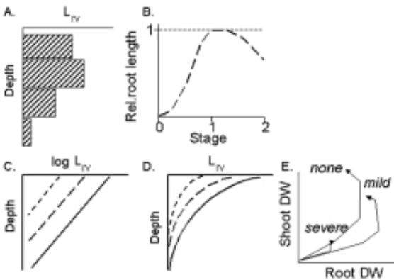
Figure 3.16. Distribution and development of crop root length density; A. Arbitrarily set values of maximum Lrv per depth interval ( Rt\_ACType = 0 ); B. multiplier to derive daily actual Lrv from maximum values per layer ( Rt\_ACType = 0 and 1); C. Exponential decrease of Lrv with depth (on log scale), D. idem (linear scale) ( Rt\_ACType = 1 ); E. Relationship between shoot and root dry weight under no, mild and severe water or N stress ( Rt\_ACType = 2 )
