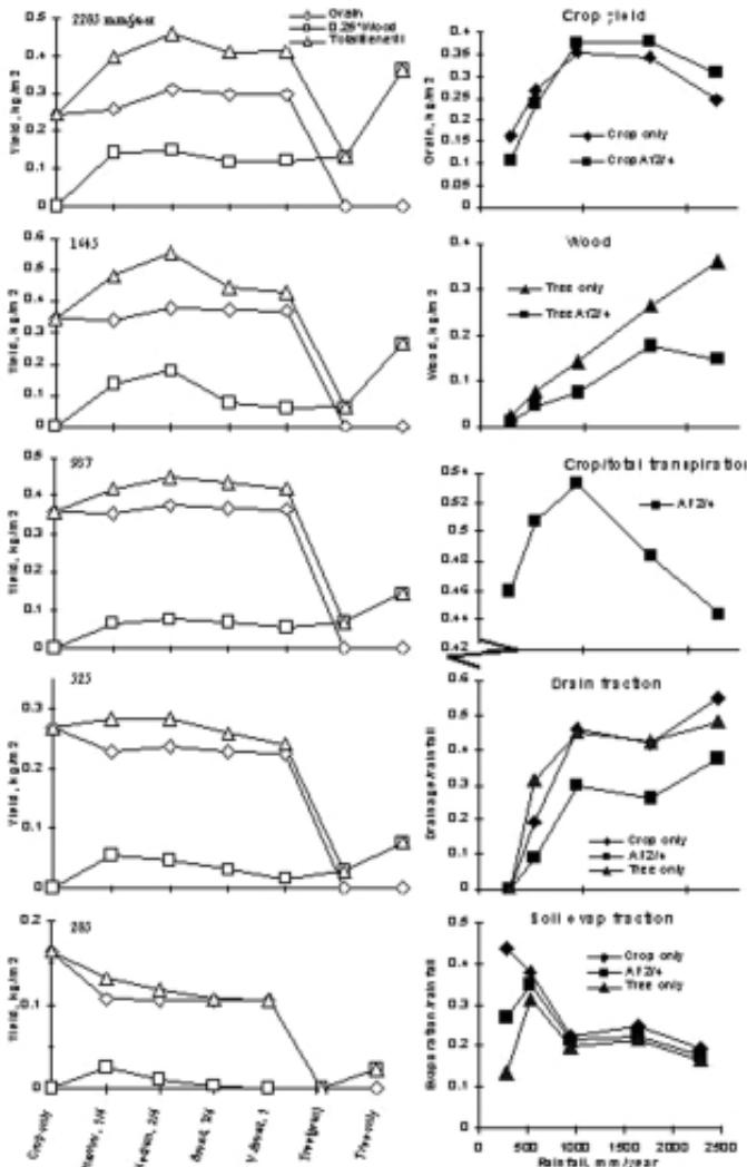
Figure 4.8 Calculations with the WaNuLICAS model of grain and wood production and water use for a range of annual rainfall conditions in an agroforestry system with isolated trees which are pruned when a crop is sown, resembling an early stage of a parkland system; production is accumulated over 2 years, involving 4 (at 2285 and 1645 mm/year) or 2 crops of 98 days duration, on a sandy soil with limited N mineralization from soil organic matter (for main parameter settings see text)
