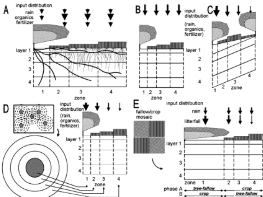
Figure 3.1 General lay out of zones and layers in the WaNuLICAS model (A) and applications to four types of agroforestry system: B. Alley cropping, C. Contour hedgerows on slopes, with variable topsoil depth, D. Parkland systems, with a circular geometry around individual trees, E. Fallow-crop mosaics with border effects.
