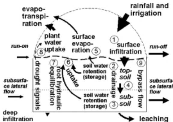
Figure 3.5. Elements of the water balance included in the WaNuLCAS model: 1. surface infiltration of rainfall, 2-4. Redistribution of water and solutes over the profile, recharging soil water content (2) and draining (leaching) excess water from the bottom of the profile, 5. surface evaporation, 6. water uptake by tree and crop roots, 7. hydraulic equilibration via tree roots, 8. drought signals influencing shoot:root allocation and 9. bypass flow of solutes.
