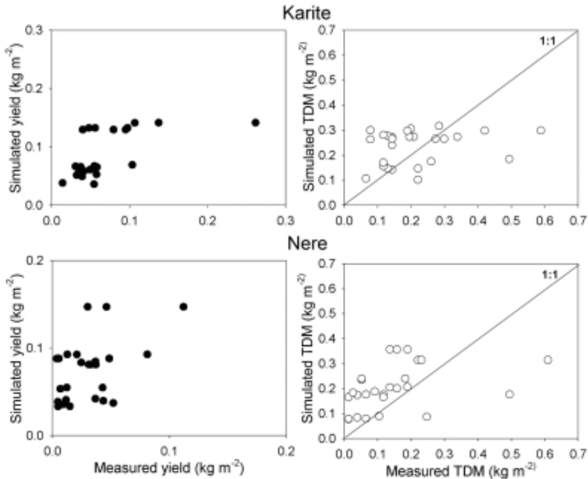
Figure 4.13 Scatter plots of measured and simulated crop yield and total dry matter (TDM) under karité ( Vitellaria paradoxa ) and néré ( Parkia biglobosa ) trees in a parkland agroforestry system in Saponé, Burkina Faso
