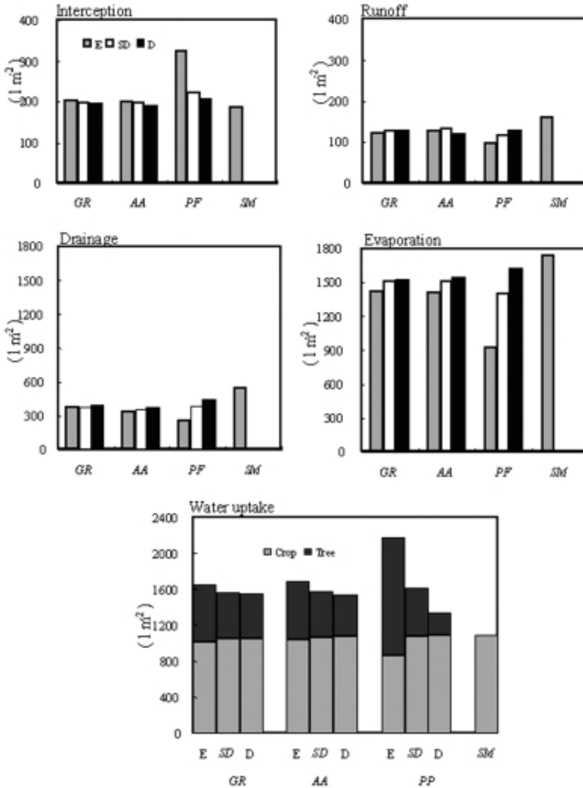
Figure 4.17 Simulated values for water balance components in (SM) sole maize and agroforestry systems containing (GR) G. robusta , (AA) A. acuminata and (PF) P. fortunei in five year simulation involving (E) evergreen, (SD) semi deciduous and (D) deciduous leaf phenology scenarios at Naro Moru
