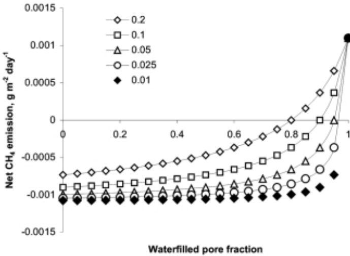
Figure 3.14. Methane flux (negative values indicate consumption, positive ones emission) as a function of the water-filled pore space, for a range of values of the GHG_CH 4 _Km parameter (a dimension parameter relating to the difference in water-filled pore space (by decrease from fully saturated soil) that causes a 50% change in net emission, within the range defined by highest and lowest flux
