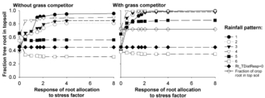
Figure 4.21 Relative tree root biomass in the upper 25 cm of the soil profile for a range of values of the factor that governs the response to stress of the biomass allocation to roots, with (right) and without (left) a competing grass; the grass is assumed not to show a functional or local response, so it has a constant fraction of its roots in the topsoil; the line Rt\_TDistResp = 0 indicates a situation without 'local response', so the 'response to stress' can modify total root biomass, but not root distribution for this setting.
