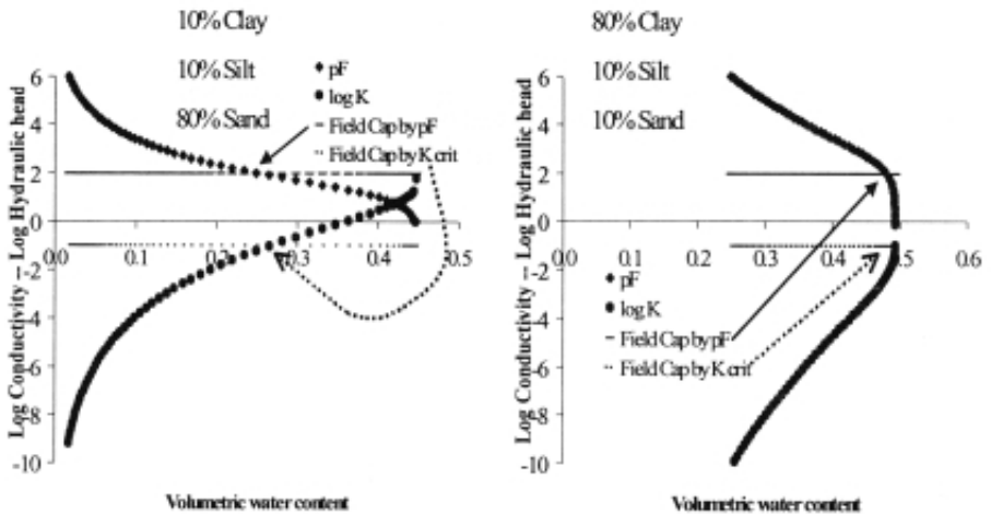
Figure 3.3. Relations between soil water content (X-axis), hydraulic head (expressed as pF or -log(head) -- positive Y axis) and unsaturated hydraulic conductivity (negative Y axis) for a sandy (left) and a clayey (right) soil, based on the pedotransfer function used in WaNuLCAS.XLS; two definitions of 'field capacity' are indicated: one based on a user-defined limiting hydraulic conductivity, and one based on a depth above a groundwater table, defining a pF value; in the model the highest value of the two for each layer and zone will be used to determine maximum soil water content after a heavy rain event
