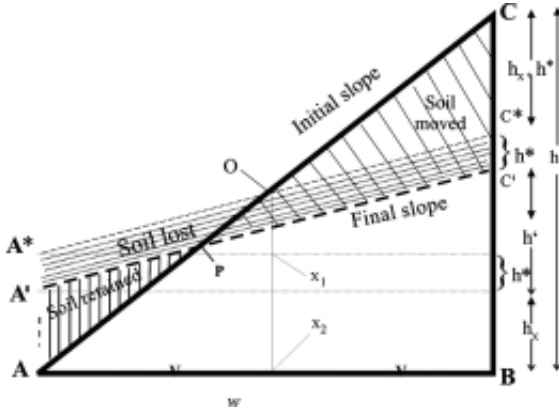
Figure 3.4. Terminology for describing change of slope: ignoring the soil below the boundary A-B which will not be affected by the changes and assuming that the bulk density of the soil is constant, the redistribution process modifies the triangle A-B-C (with a width w , a height h and a slope-length s ) into the polygon A-A'-C'-B (with height h' and slope length s' ), plus the soil loss which is proportional to AA^*C^* , or wh^* ; the triangle AA^*O is equal to OCC^*
