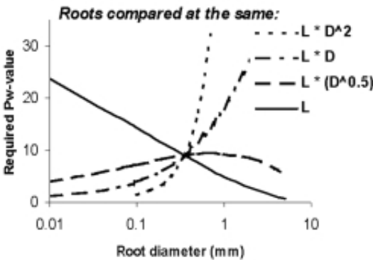
Figure 3.18. Effect of root diameter on potential uptake when root systems of different diameter are compared at equal length, root surface area or volume (weight): the smallest effect of root diameter exists when root length times the square root of the root diameter is used (Van Noordwijk and Brouwer, 1997)
