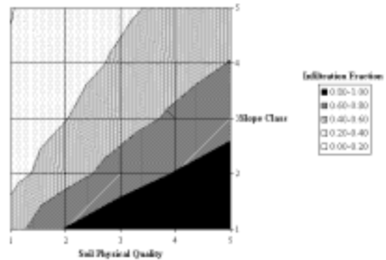
Figure 2. Infiltration fraction of a plot depending on slope and soil physical quality; slope is classified according to USLE (1: slope < 1%, 2: 1% ≤ slope < 3%, 3: 3% ≤ slope < 5%, 4: 5% ≤ slope < 20%, 5: slope > 20%); where soil physical quality represents its aggregate stability.
