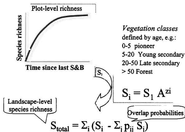
Fig. 2. Relations used for deriving total species richness of the landscape, S_{\text{total}} , on the basis of the species richness of each plot (related to its age since the last S&B event), and the allometric scaling rules for species richness within each land cover class (based on its area A and the scaling parameter z_i ) and the overlap matrix p_{ij} between land cover types.
